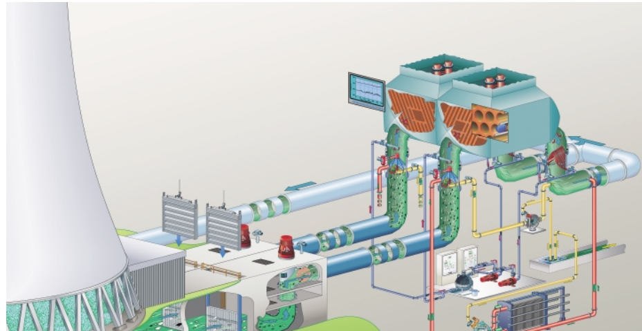
TAPROGGE in power stations with cooling towers
