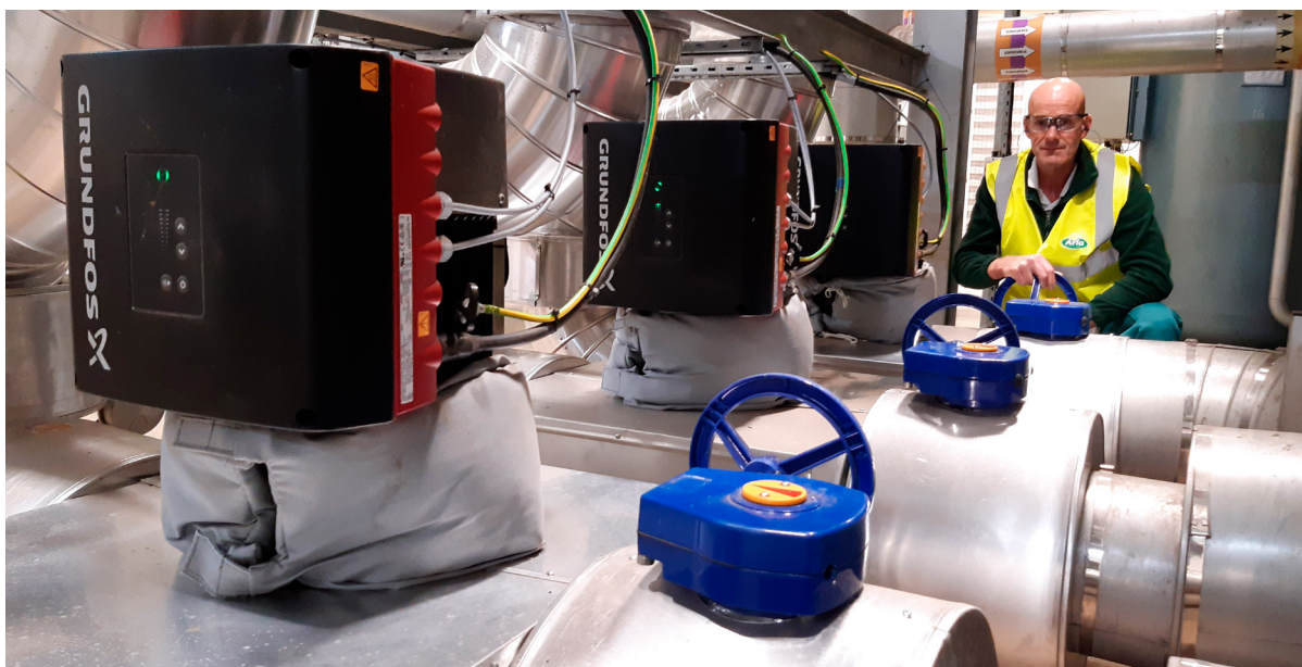
Figure 5: Intelligent control modes ensure secure integration of NKE and NBE standard pumps and end suction pumps, for example, with TPE inline pumps in cooling water circuits.
